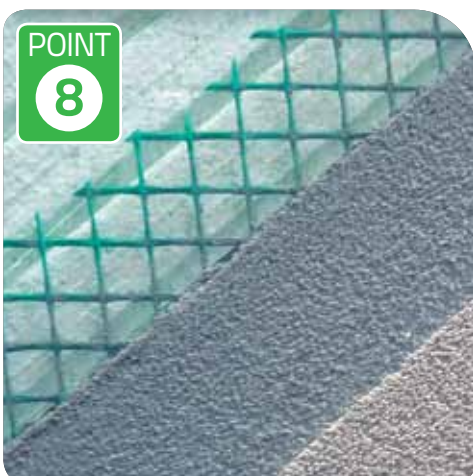
Reinforced Fibreglass Mesh ▪ Trowelled into a 1st Coat Render
